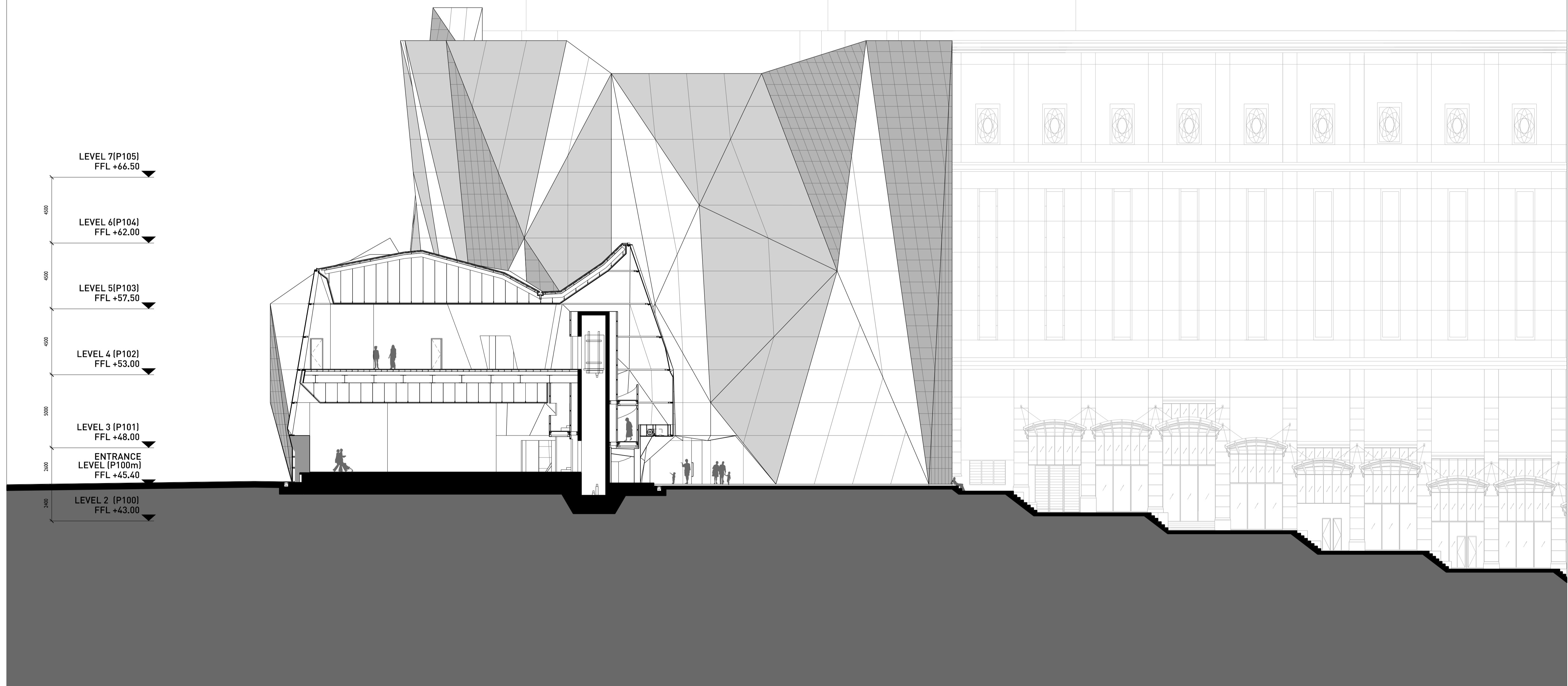
1 SECTION THROUGH PAVILION GA/s204 SCALE 1:150
