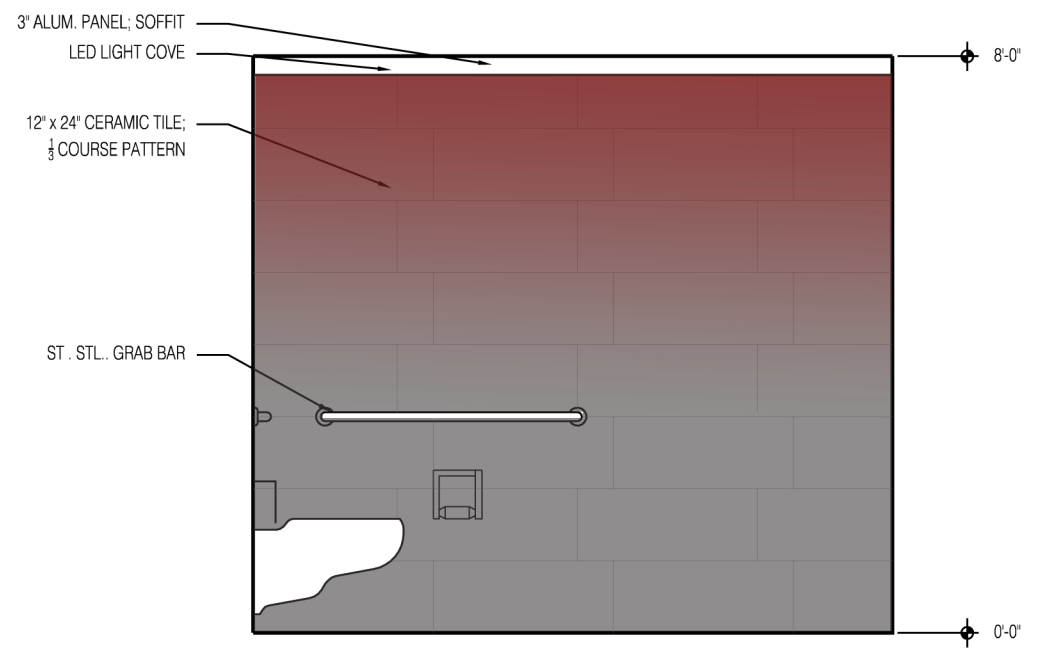
B.1:CFI-9.4 SOUTH ELEVATION 3/8" = 1'-0"
