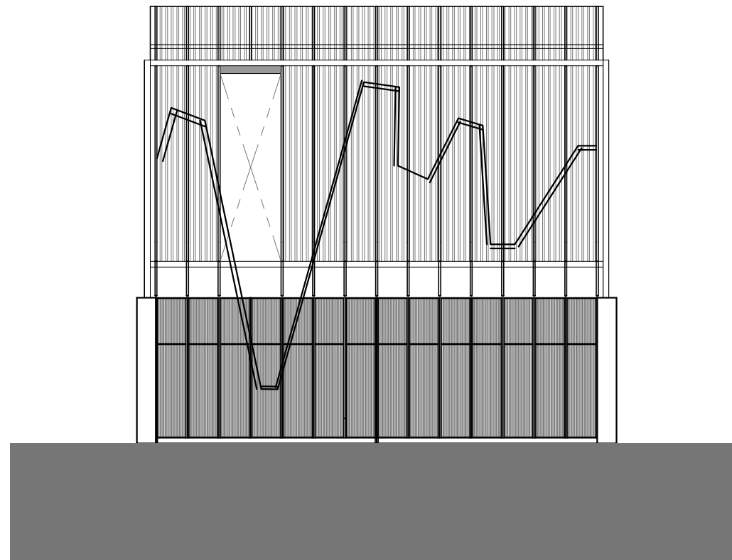
SOUTH ELEVATION
