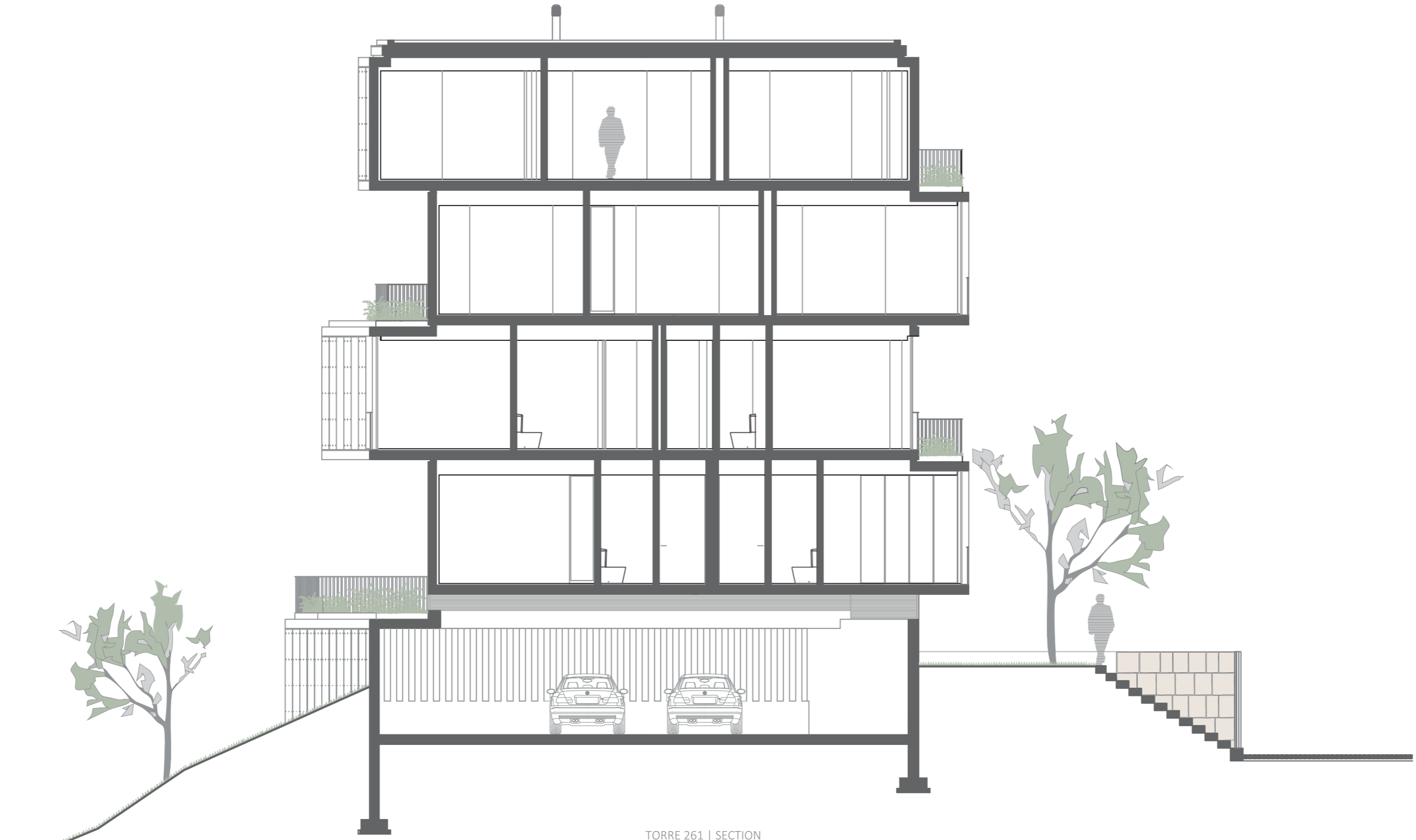
TORRE 261 | SECTION
