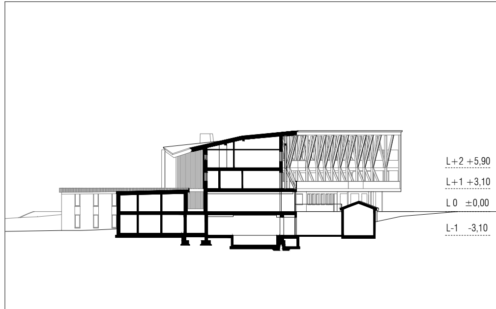
SECTION
