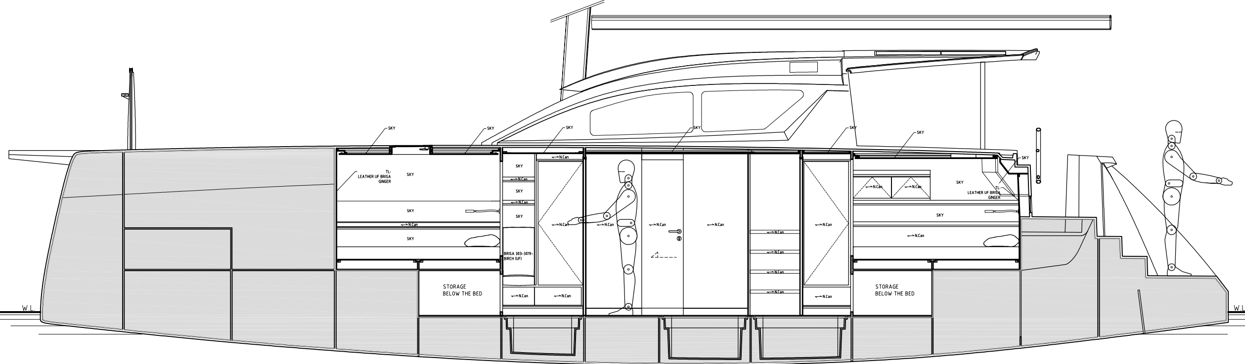
SECTION Y-Y
