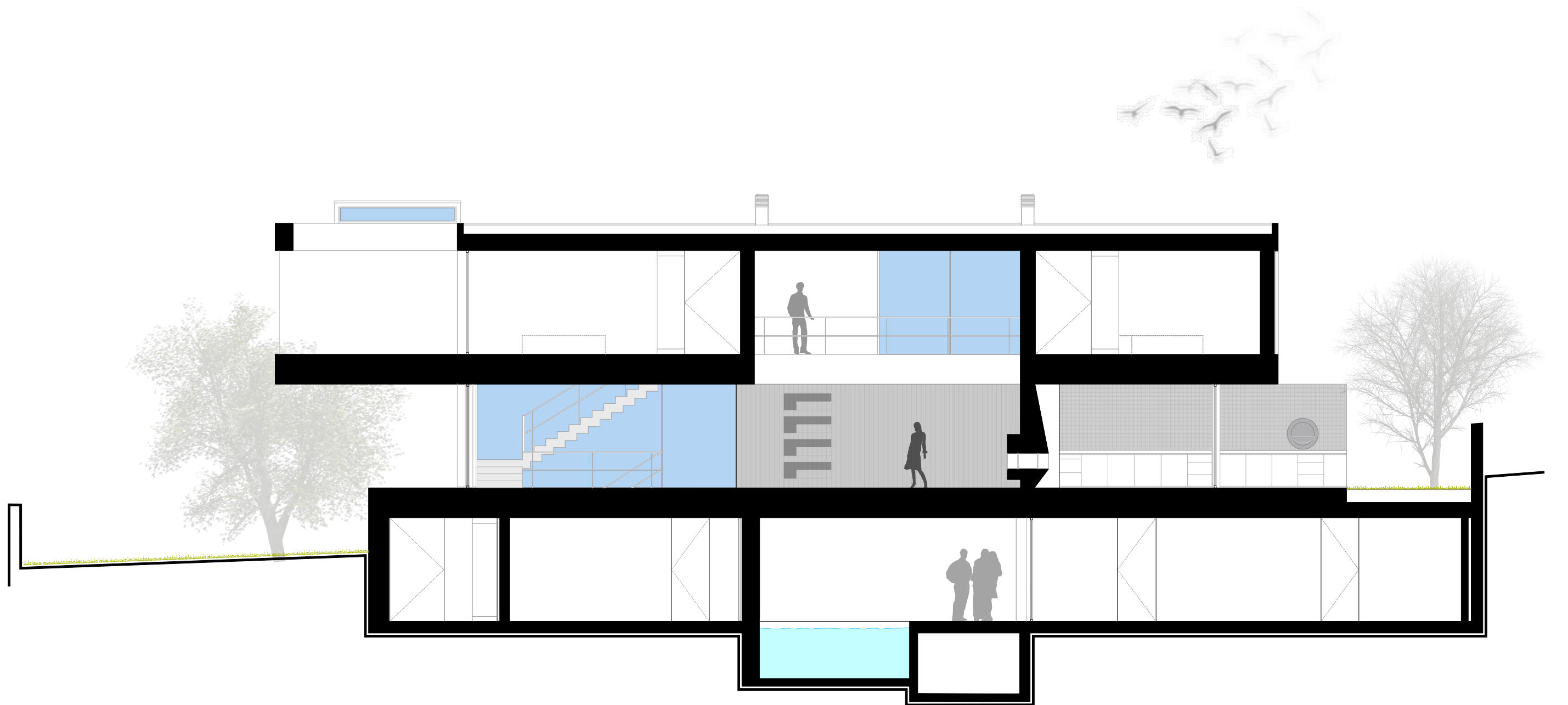
Section S1
