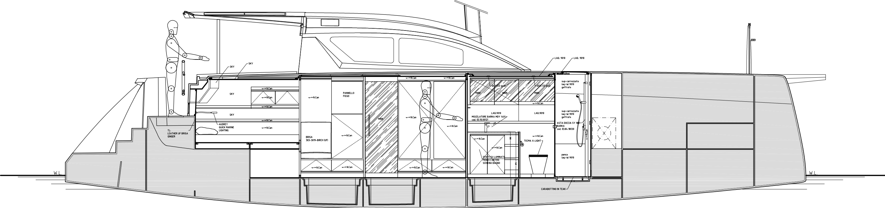
SECTION Q-Q
