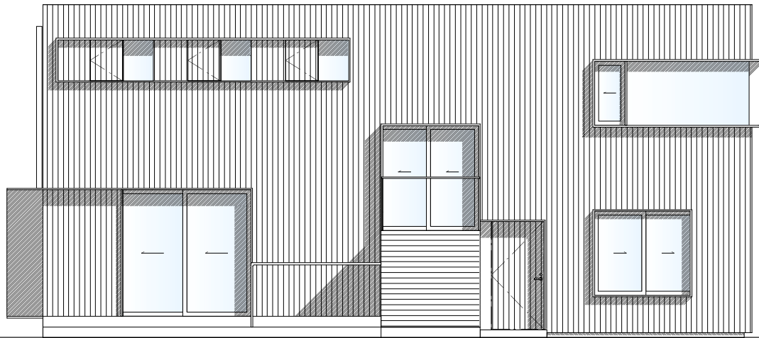
South Elevation
