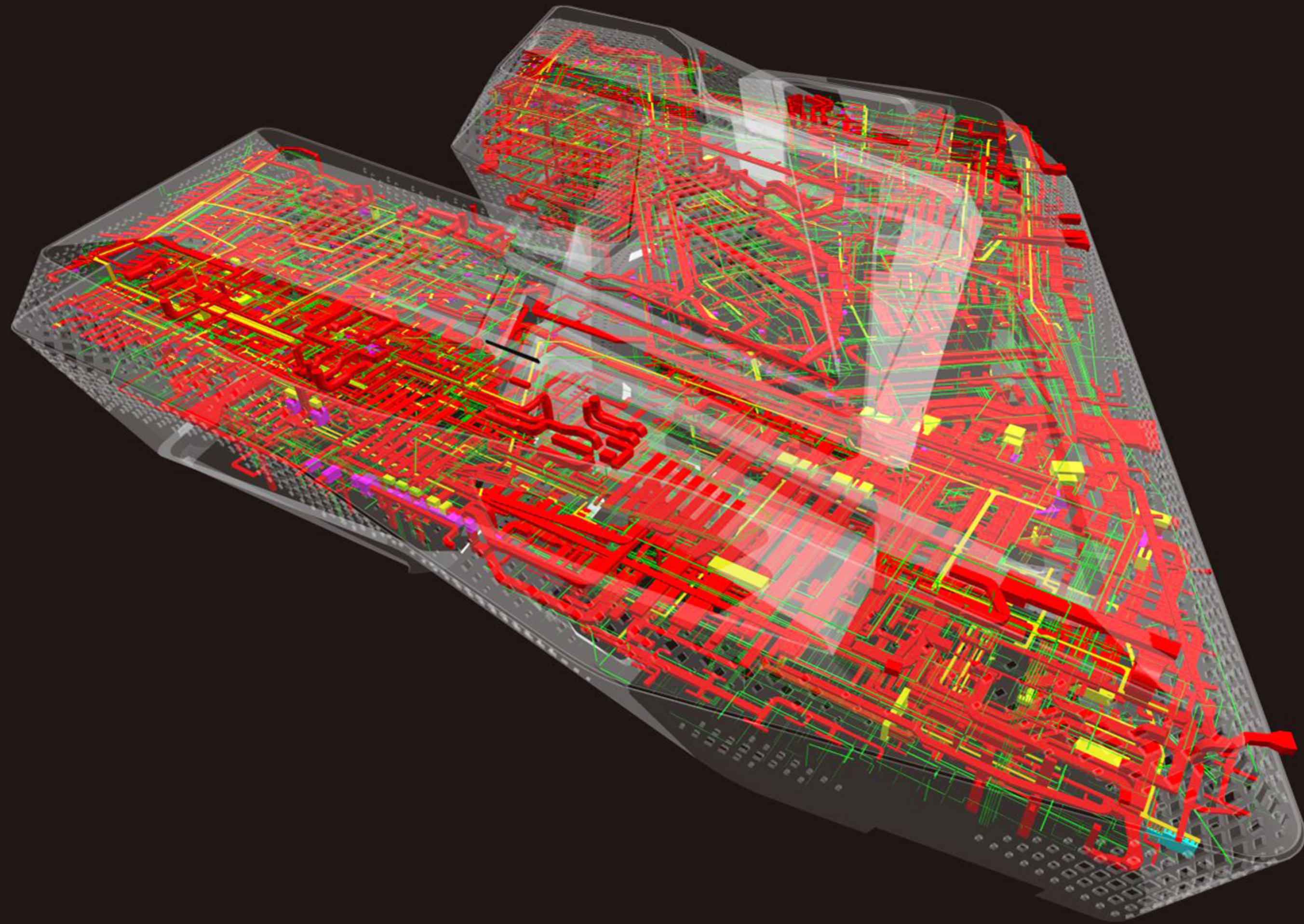
Nanjing International Youth Cultural Centre BIM MODEL - MEP
