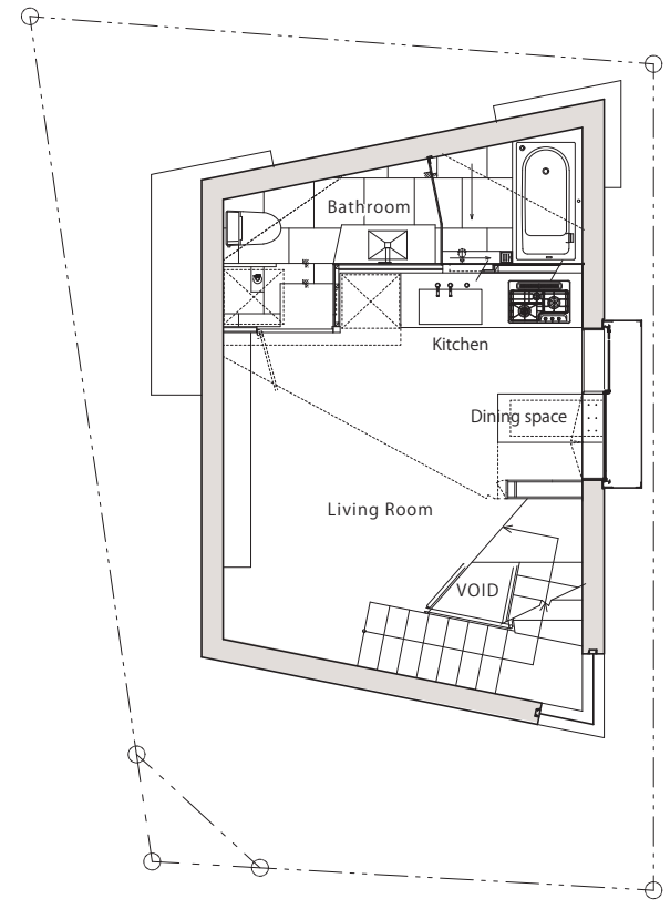
2nd Floor S=1/100
