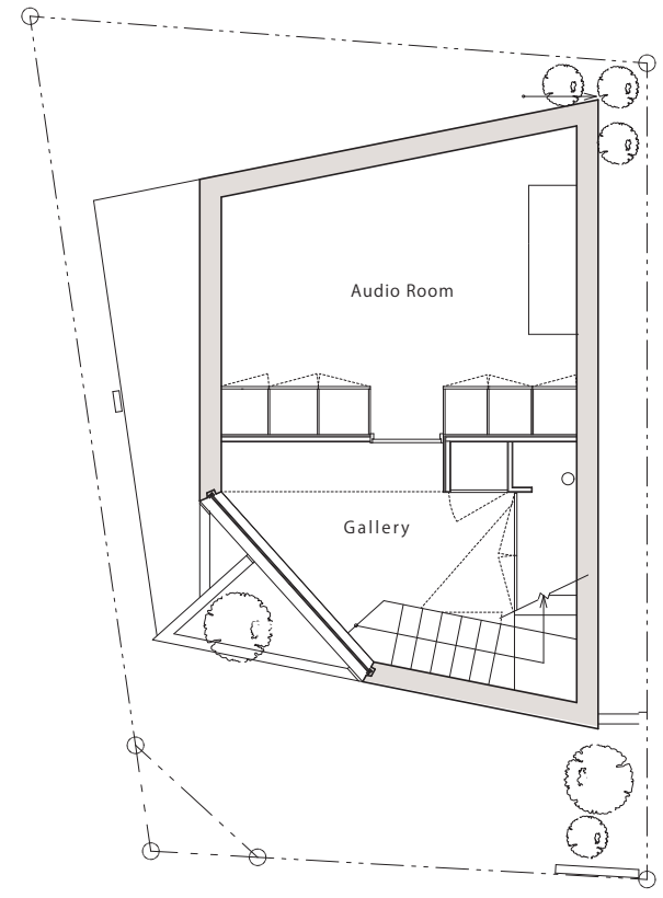
Underground Floor S=1/100
