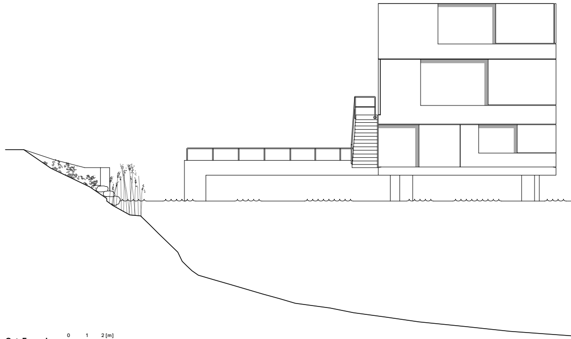
Ost-Fassade 0 1 2 [m]
