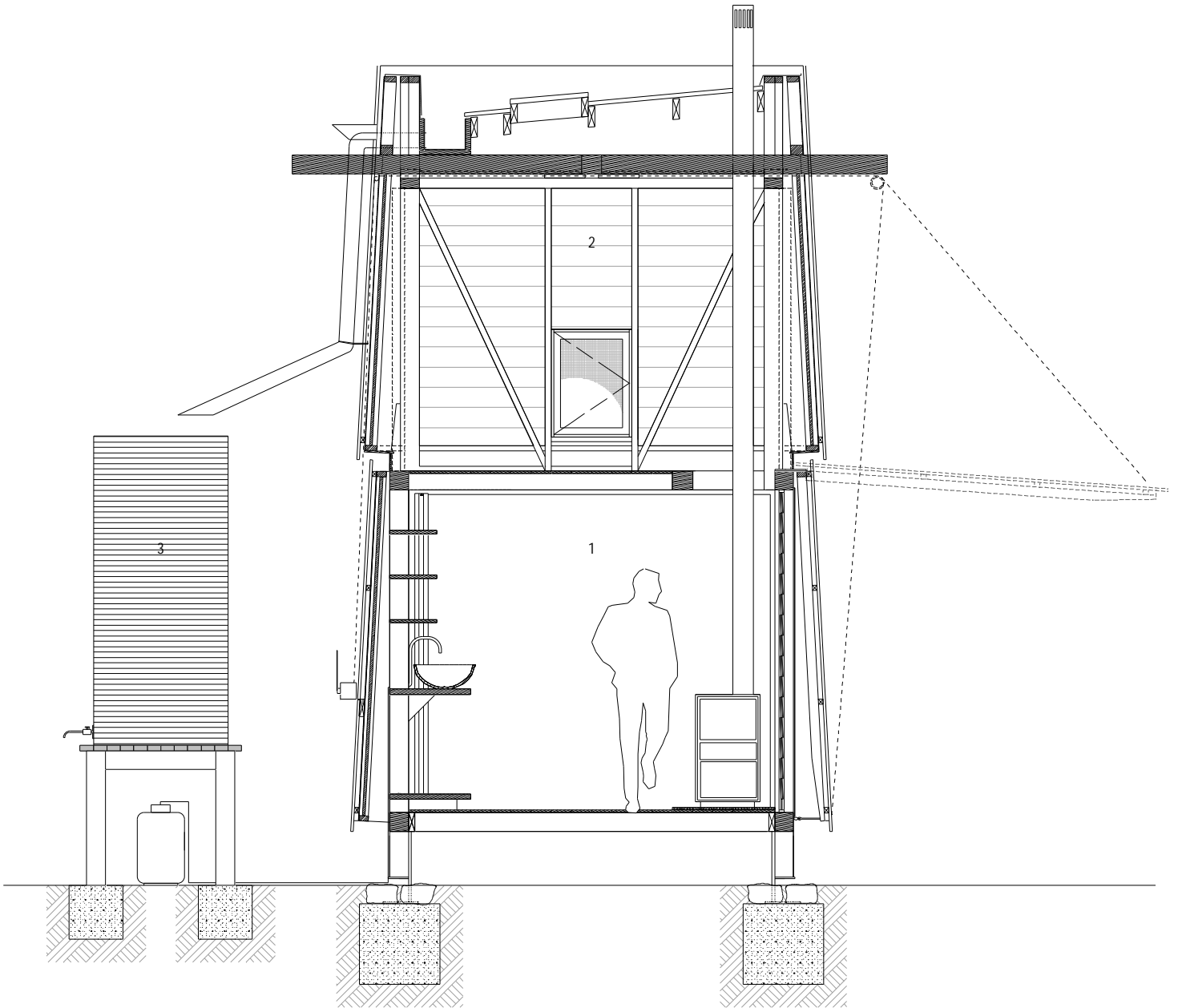
Permanent Camping Mudgee Section 1 Living 2 Sleeping 3 Watertank
