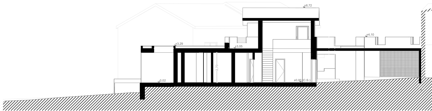
Section 1 (C1)
