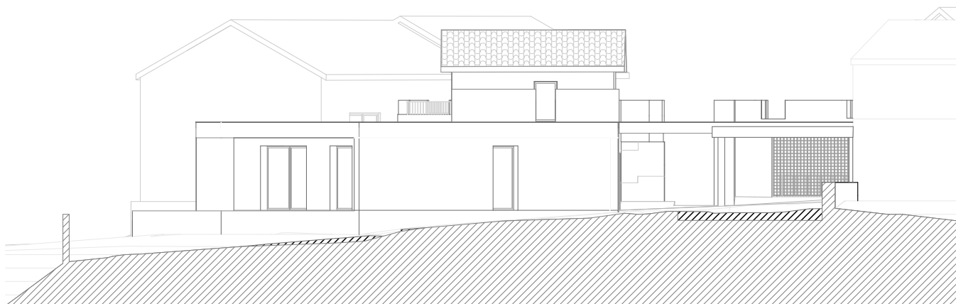
Northern elevation
