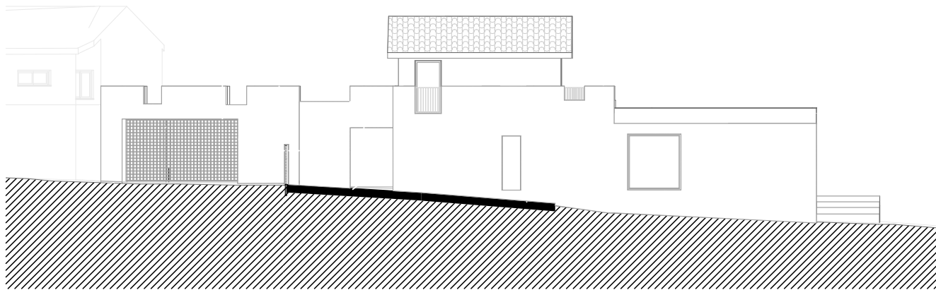
Southern elevation (frontal)
