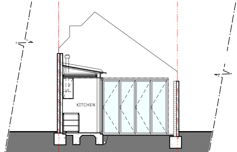
west elevation / section
