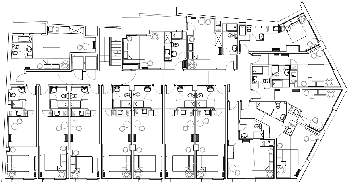
FIRST FLOOR
