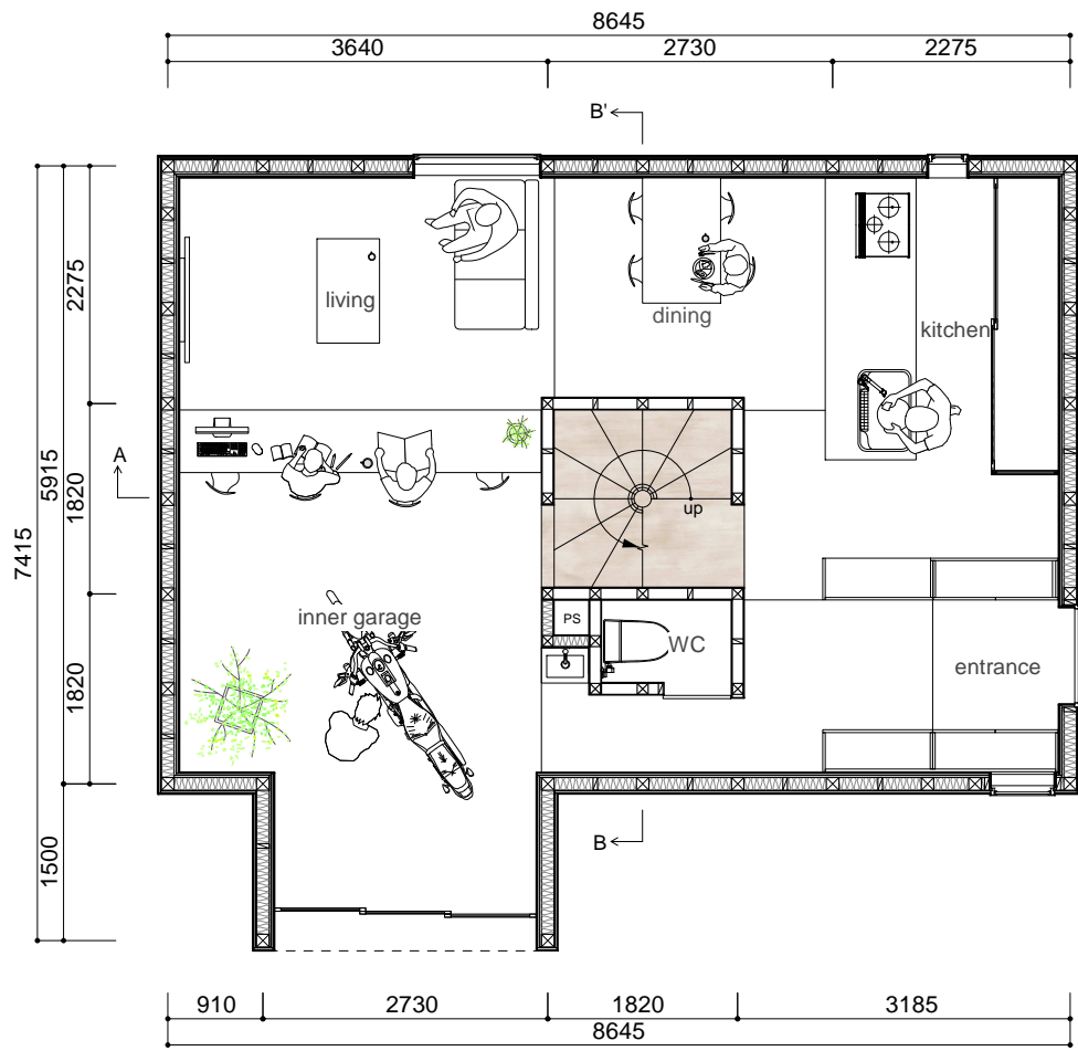
1F PLAN 1:80
