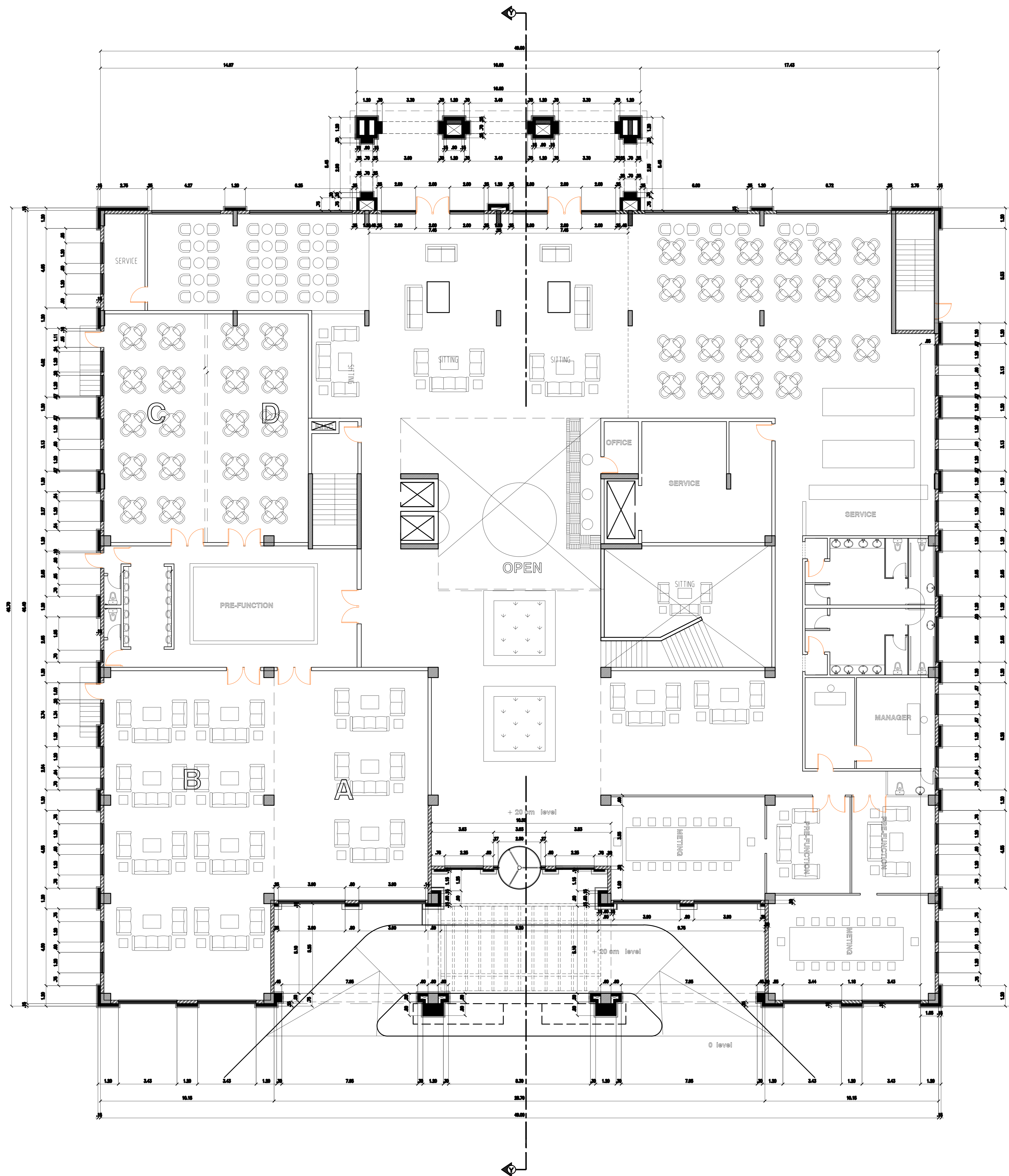
1 A3 GROUND FLOOR PLAN BUILDING -B SCALE 1:100 M
