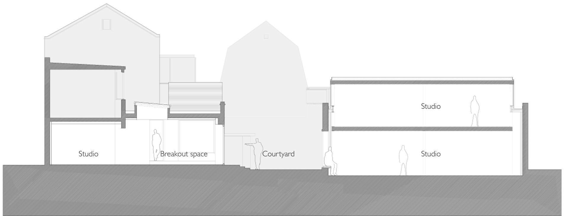
Section B-B
