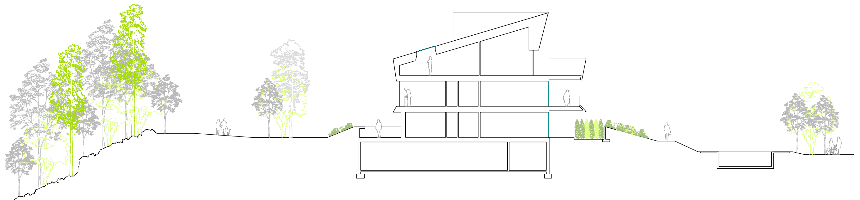
CROSS SECTION e 1_200
