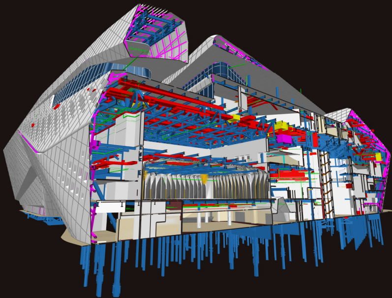
Nanjing International Youth Cultural Centre BIM MODEL - Section
