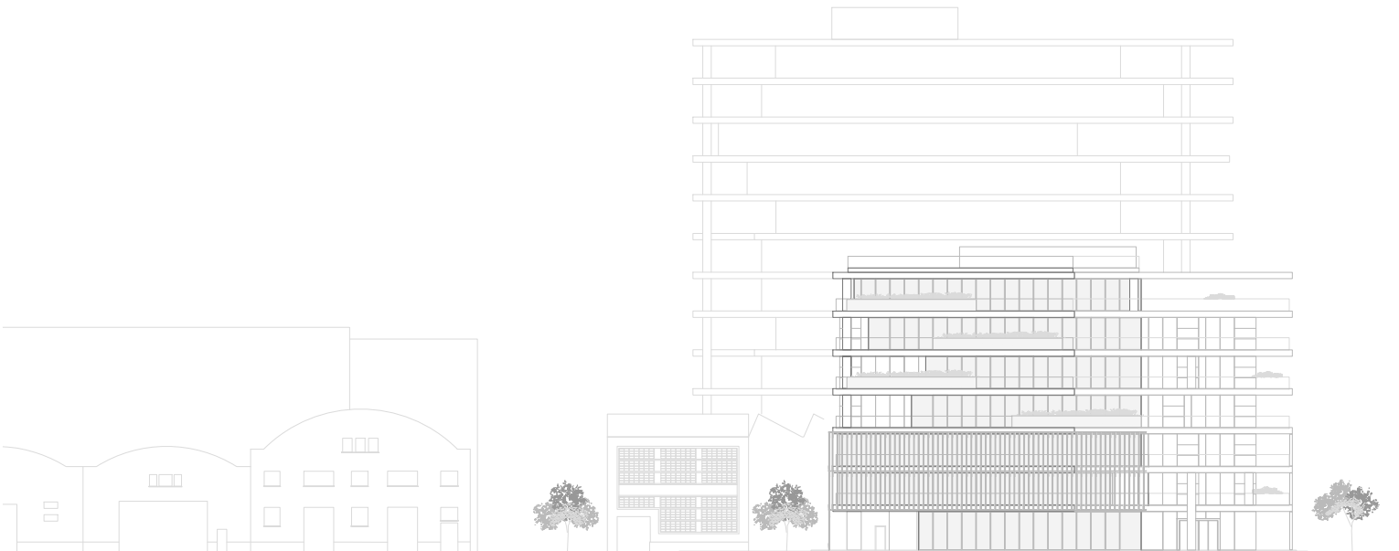
Alzado Suroeste. Southwest Elevation
