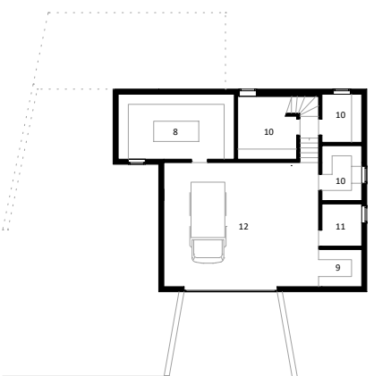
basement floor
