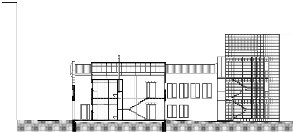
SECTION A 0 2 5
