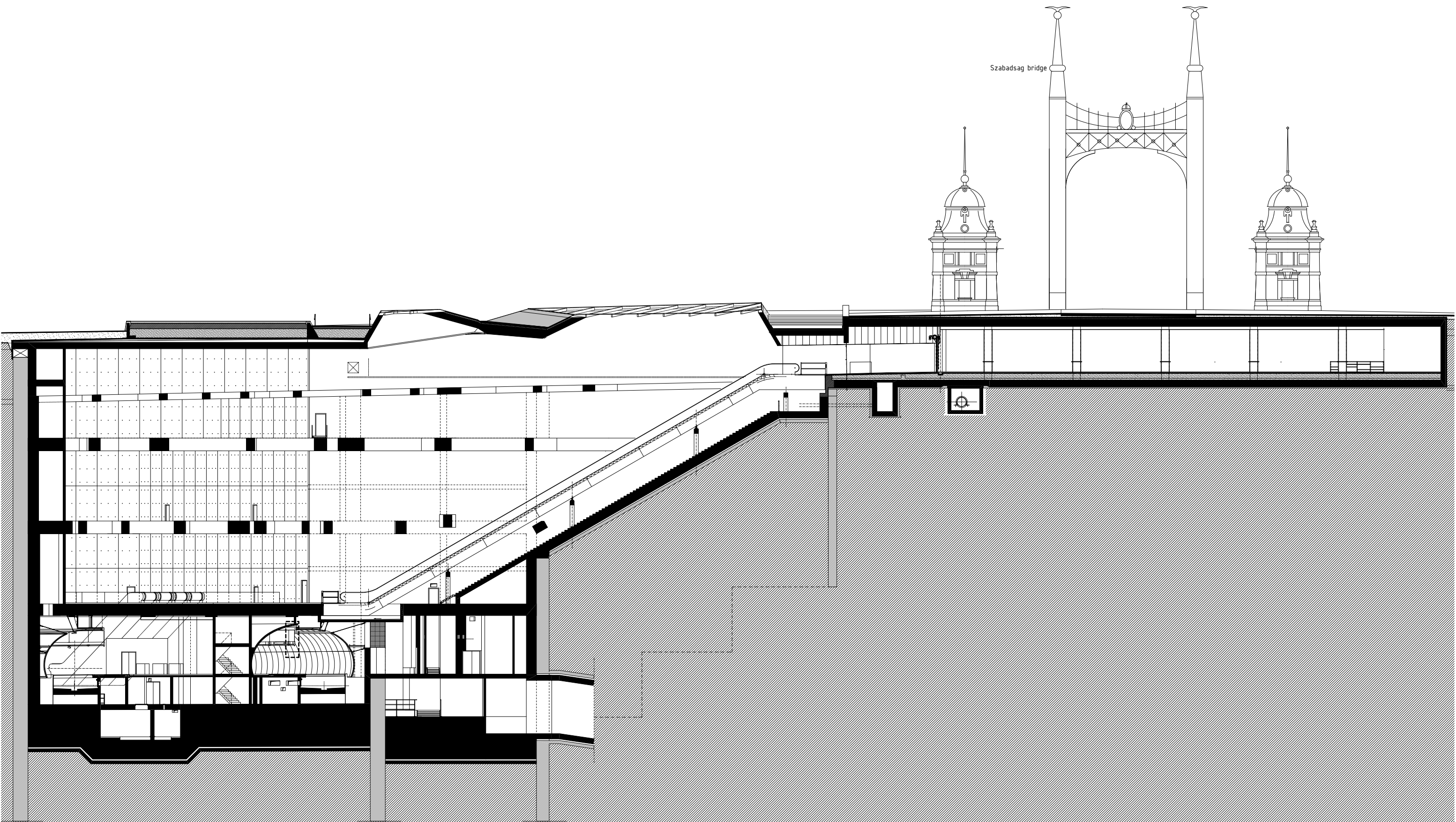
section C-C
