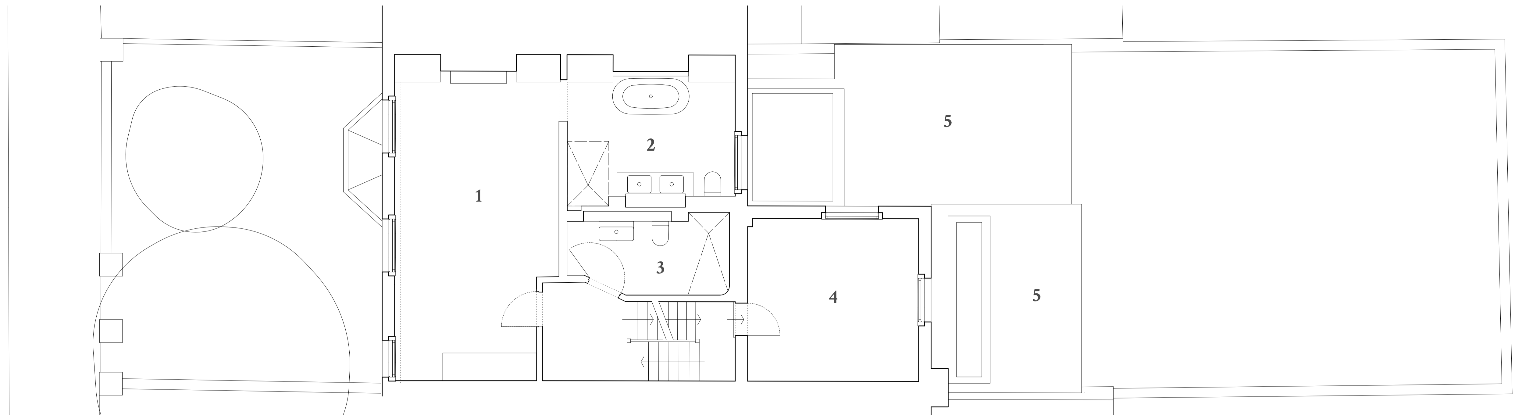
First Floor 1:50
