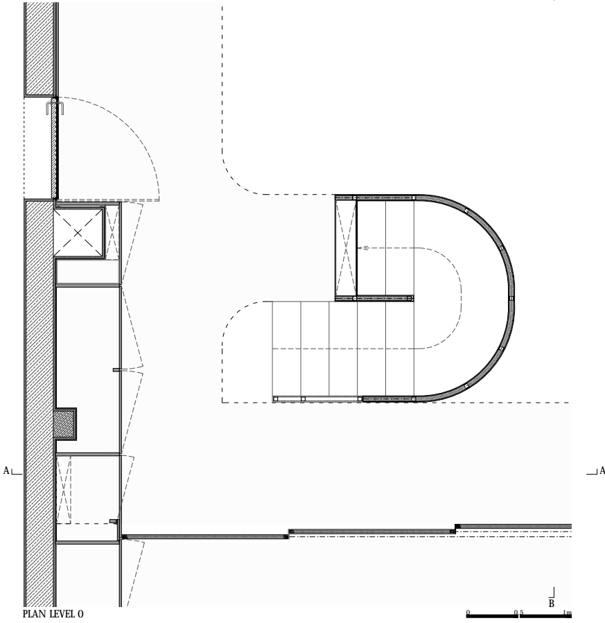
PLAN LEVEL 0
