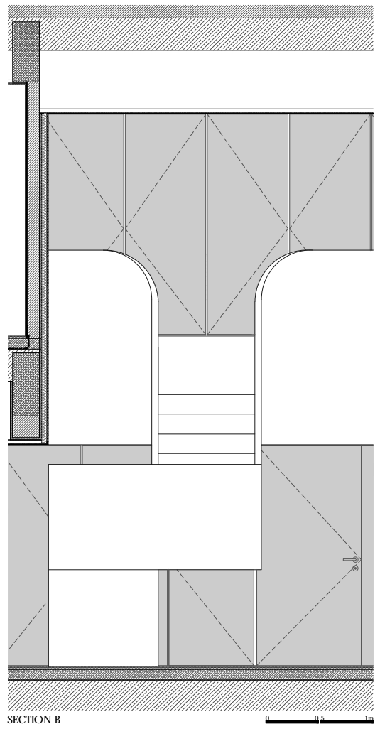
SECTION B
