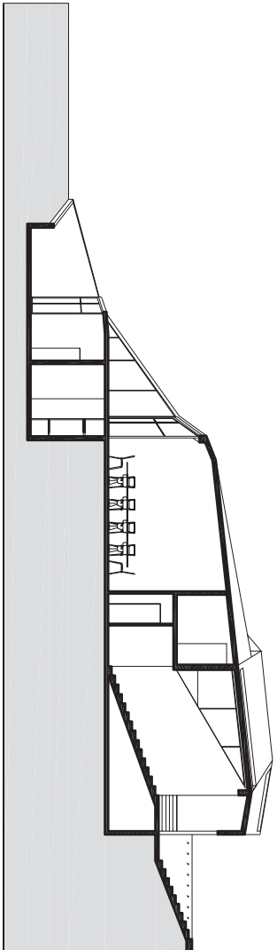
SECTION B-B'
