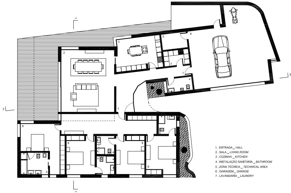
\\ PLANTA PISO 0 _ GROUND LEVEL PLAN
