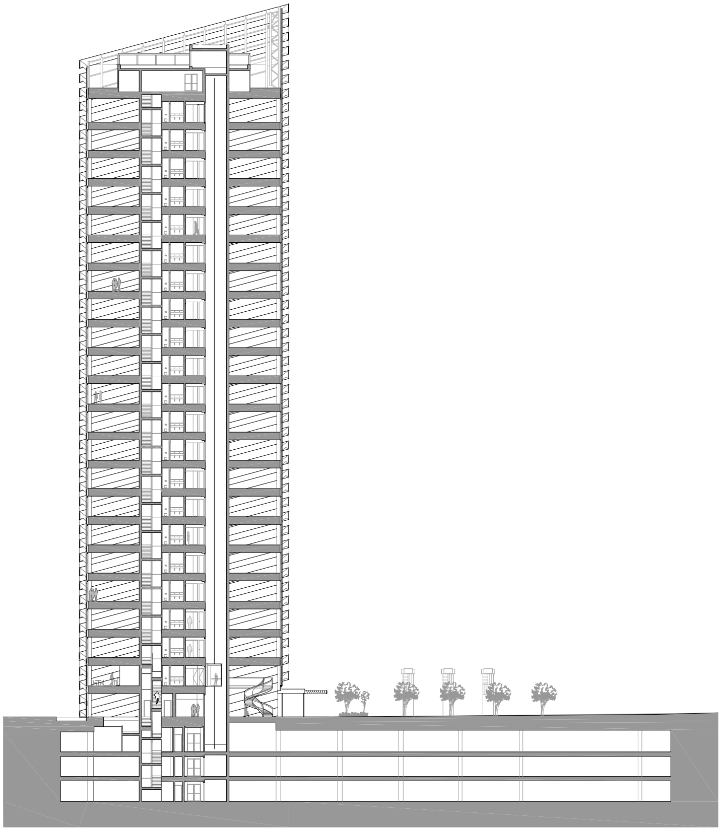
SECCION INGRESO PRINCIPAL / SECTION THROUGH MAIN ENTRANCE
