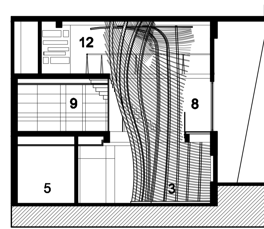
SECTION A 0 1 2 5
