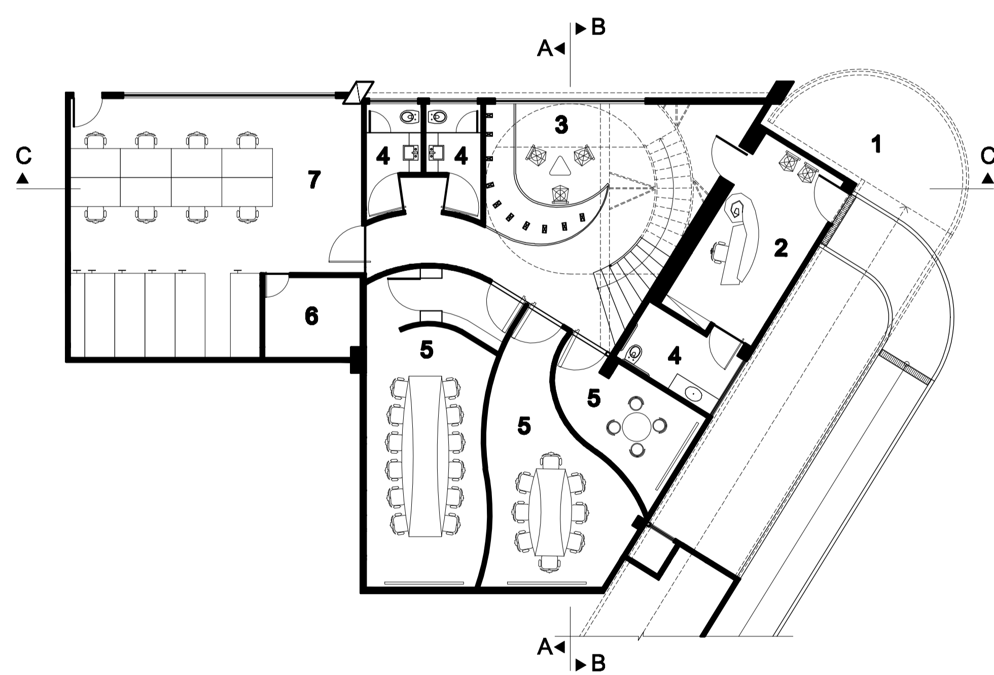
First Floor 1-Rowing stands access (ramp) 2-Reception 3-Waiting area / informal meeting 4-W.C. 5-Meeting rooms 6-Audio and Video room 7-Workstations
