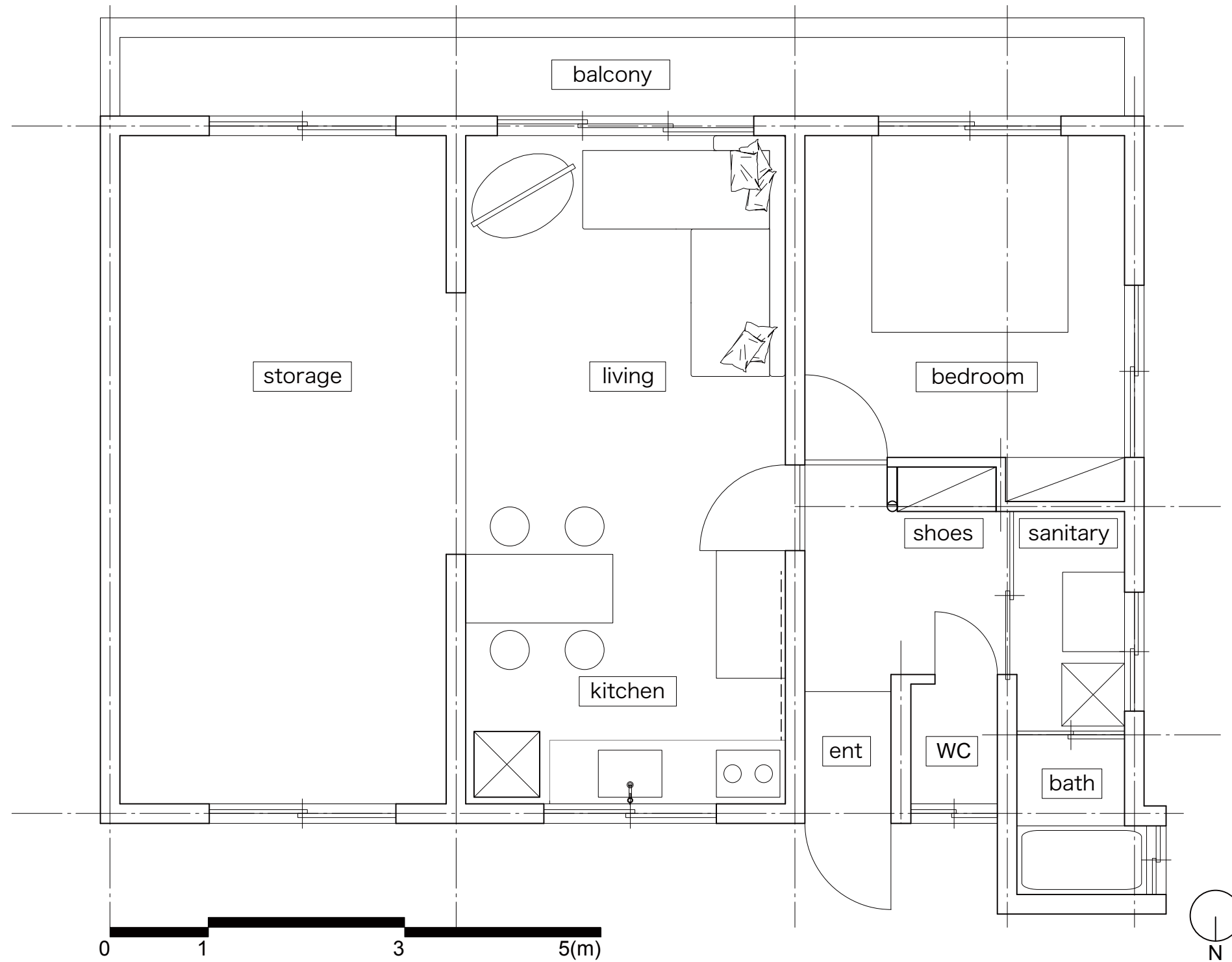
before renovation plan S=1/50
