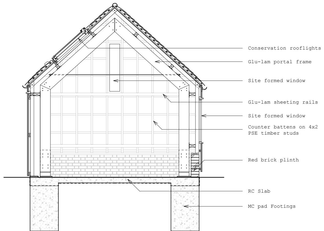
SHORT SECTION 1:50 @ A3
