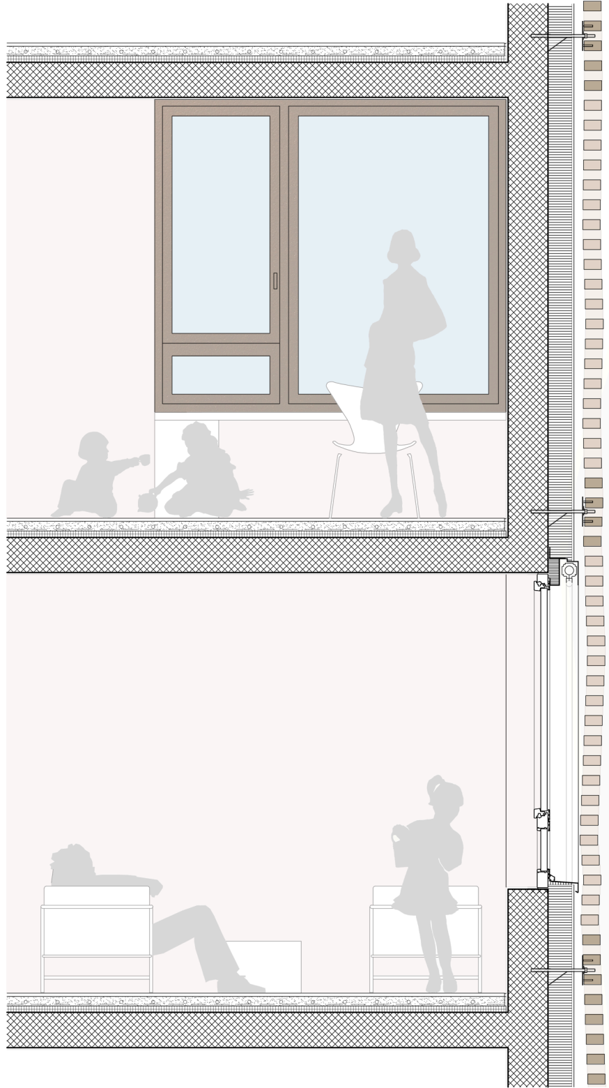
Detail plan floor and section 1:33
