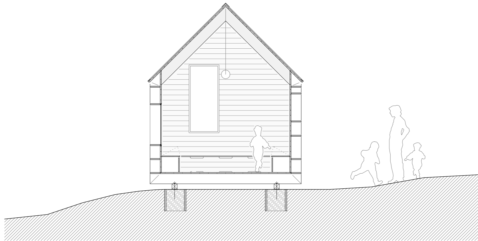
Section M 1:50 | © Bernd Riegger
