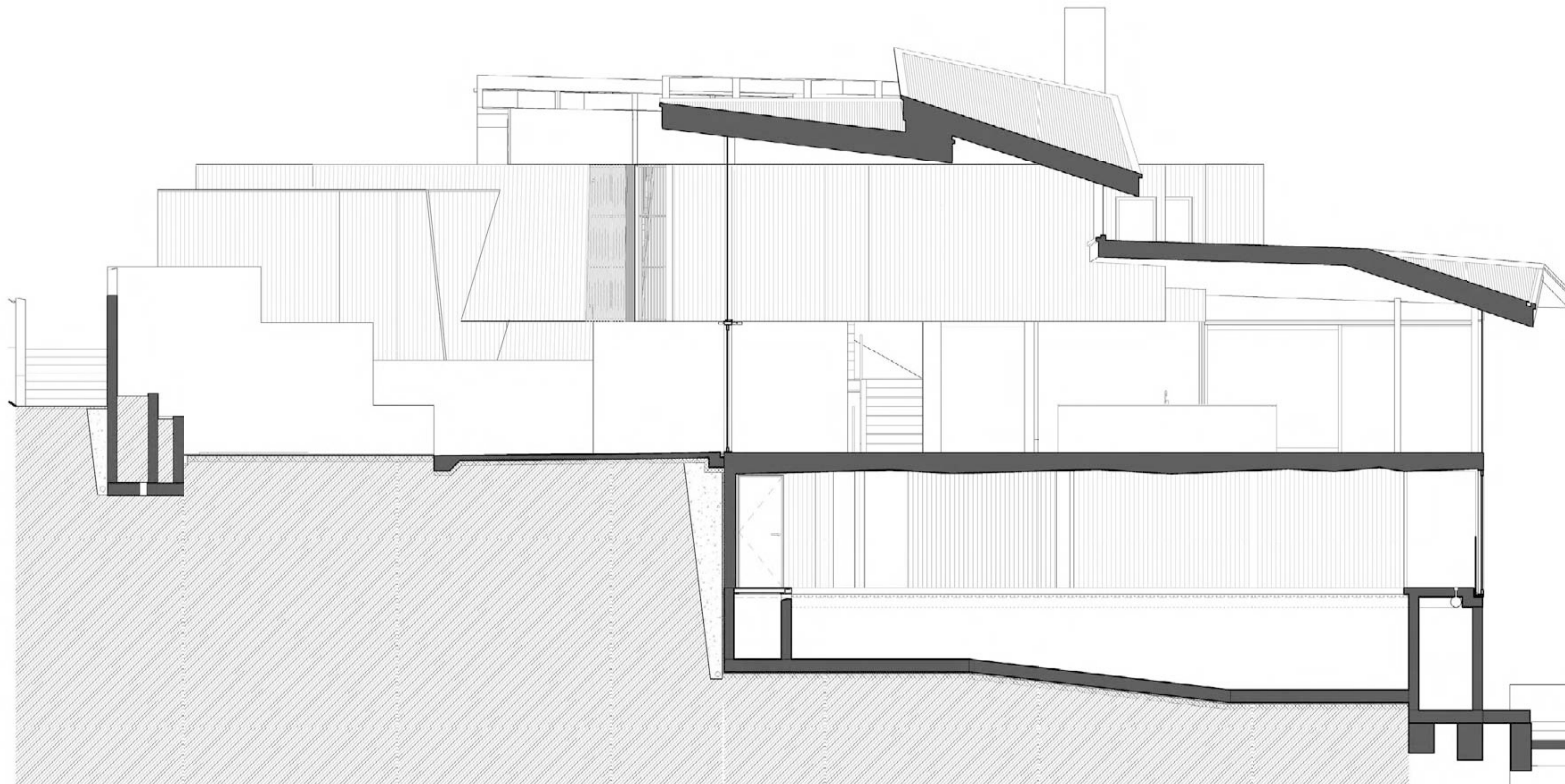
SECTION THROUGH FAMILY / KITCHEN / POOL
