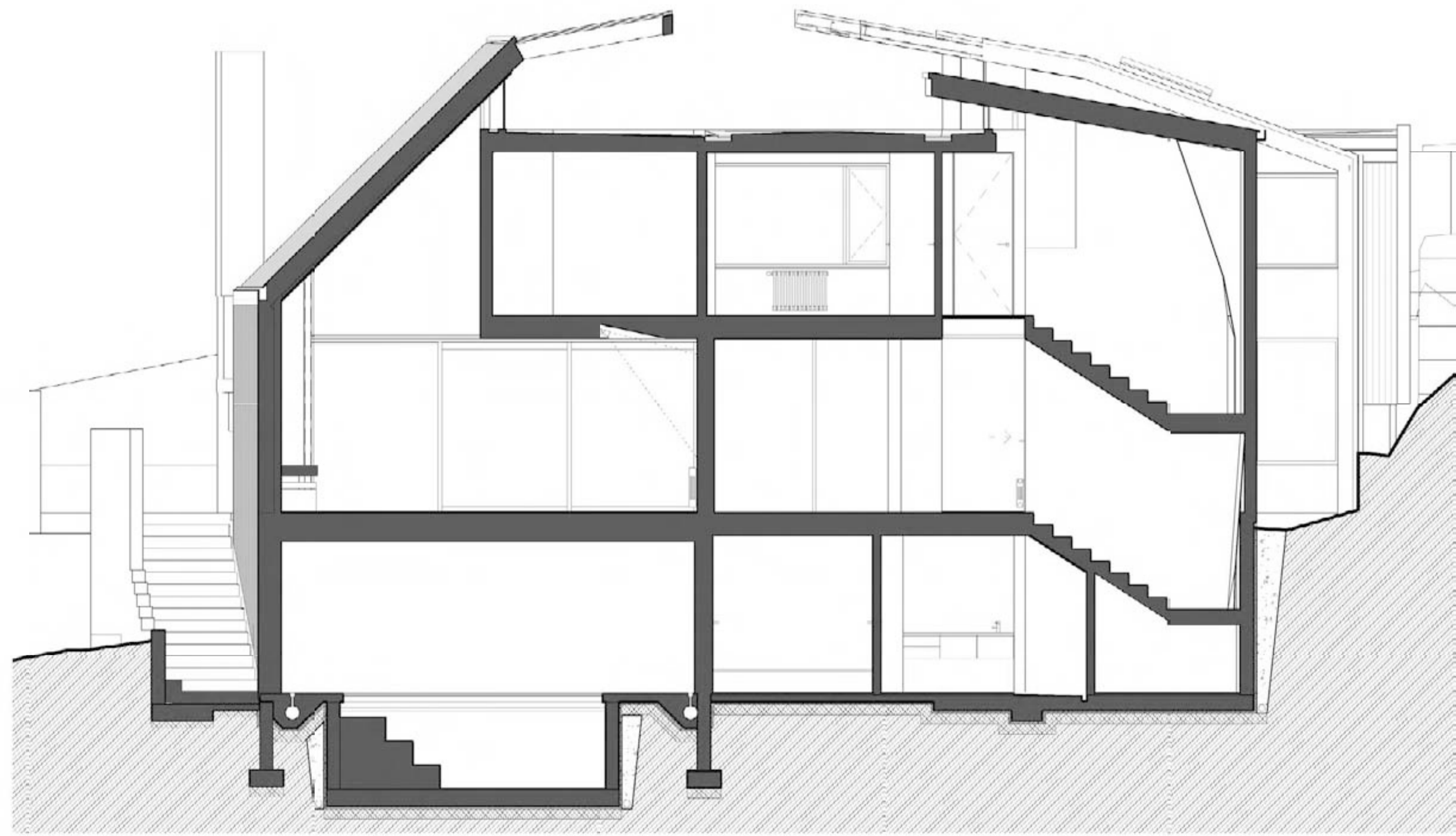
SECTION THROUGH WEST STAIR
