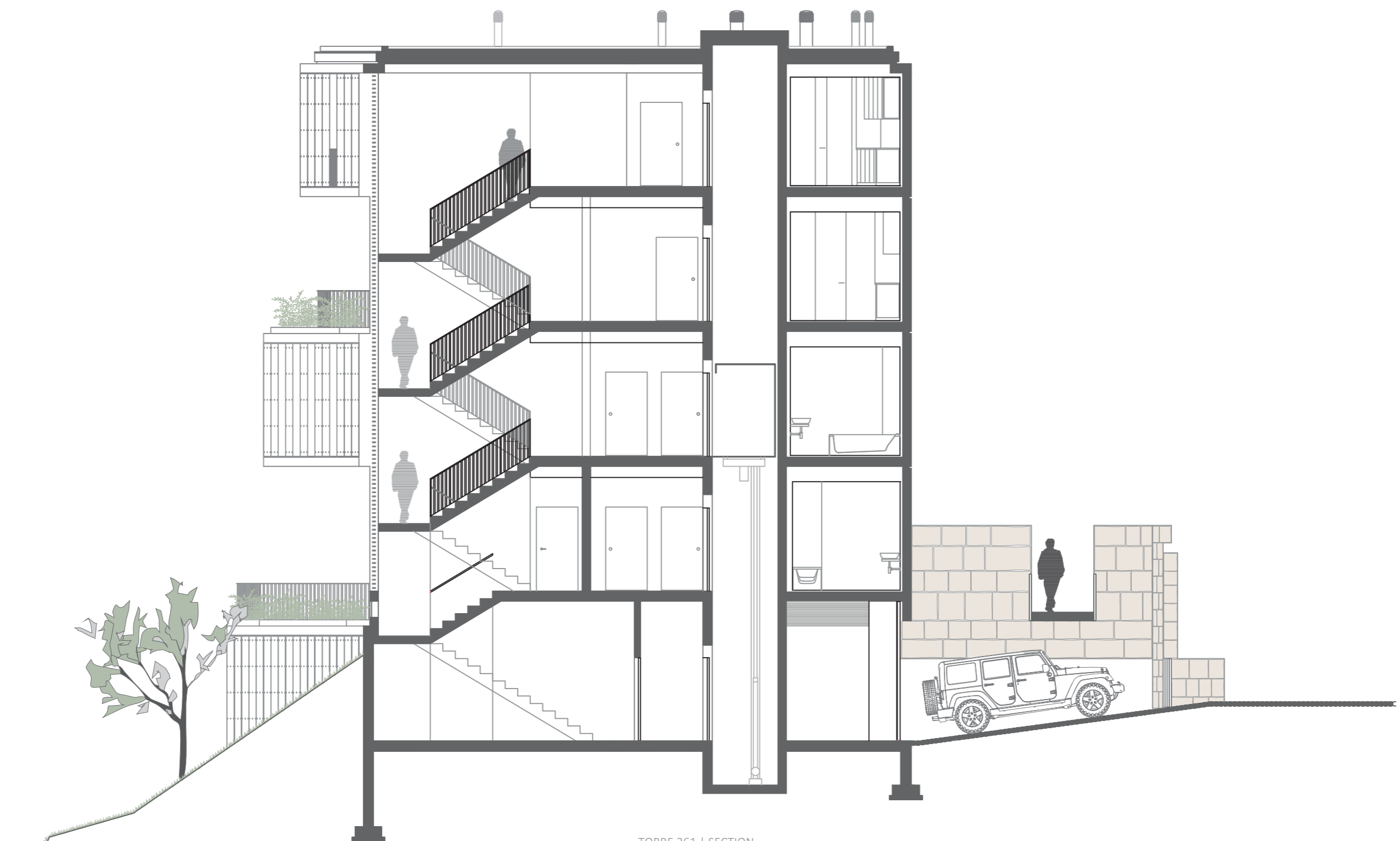
TORRE 261 | SECTION
