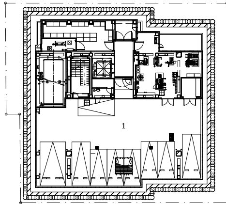
First Basement Floor plan
