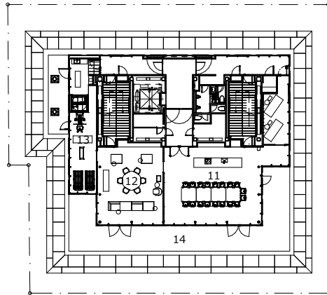
Fifth Floor plan
