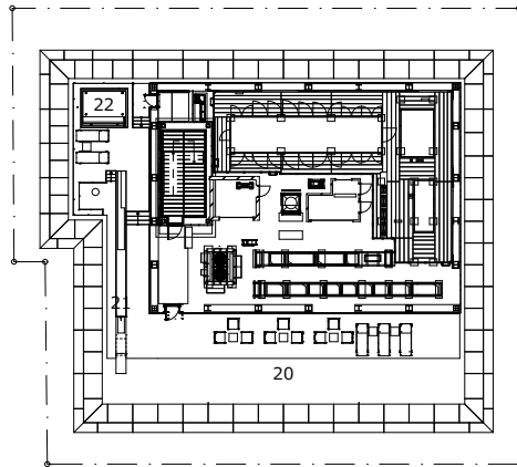
Rooftop plan
