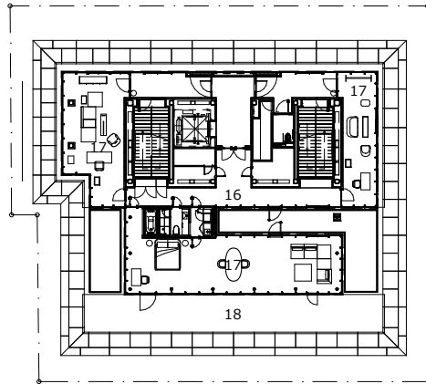
Seventh Floor plan
