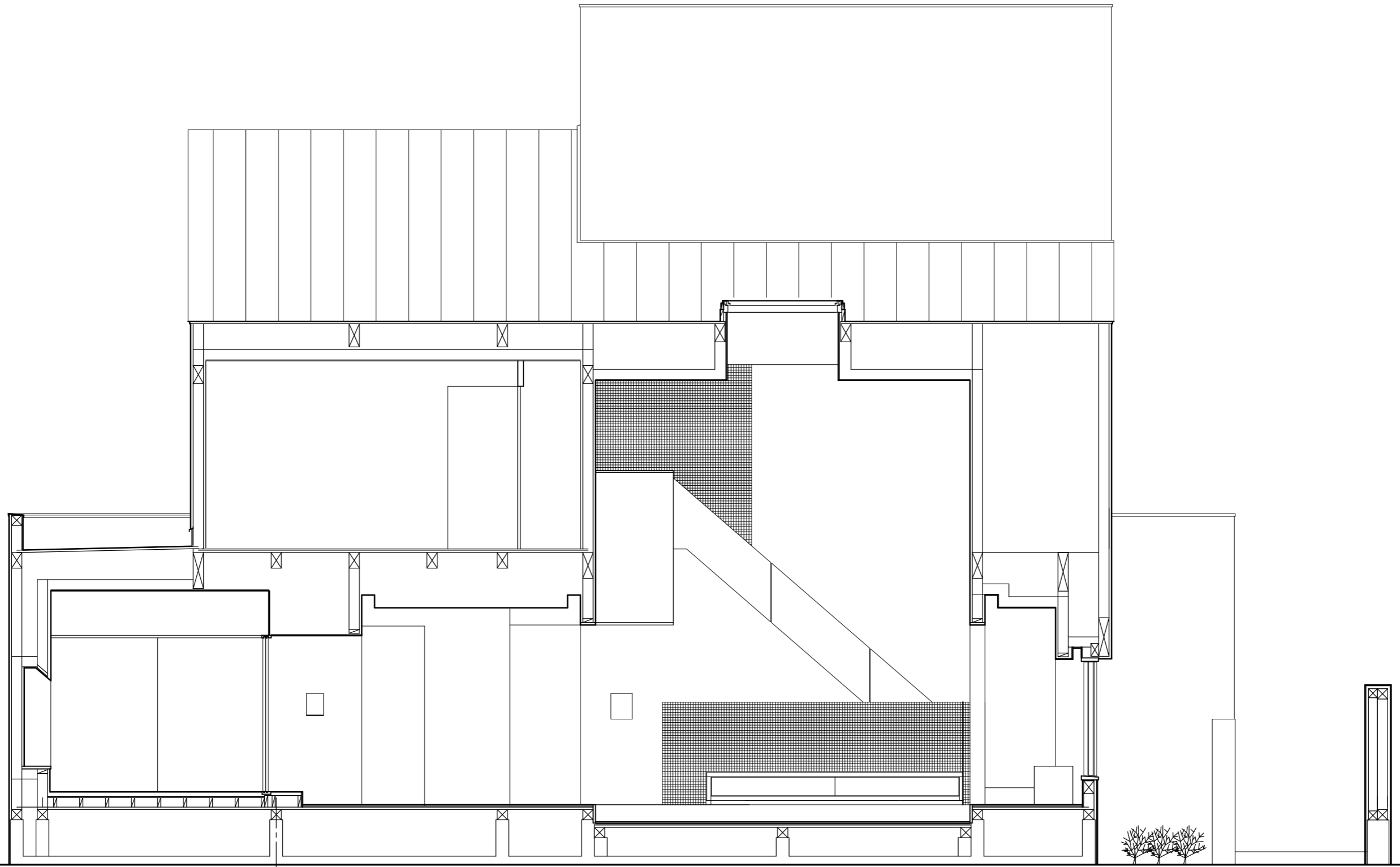
SECTION
