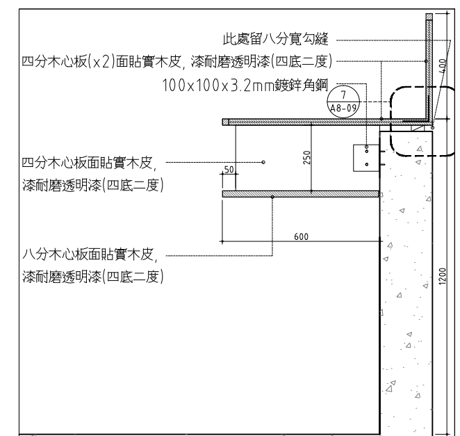
13 2/3/4F立式檢索台暨帶狀座椅 立面詳圖(檢索區) SCALE: 1/10 UNIT: mm
