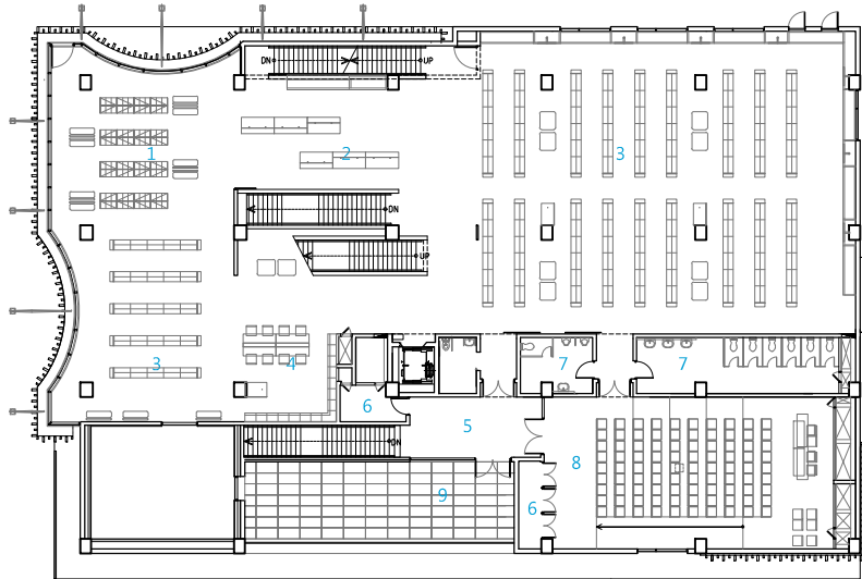
2F plan
