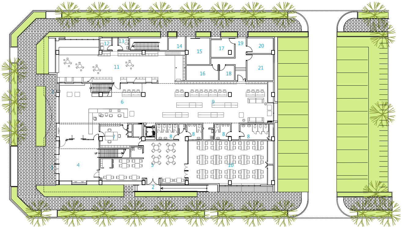
1F plan
