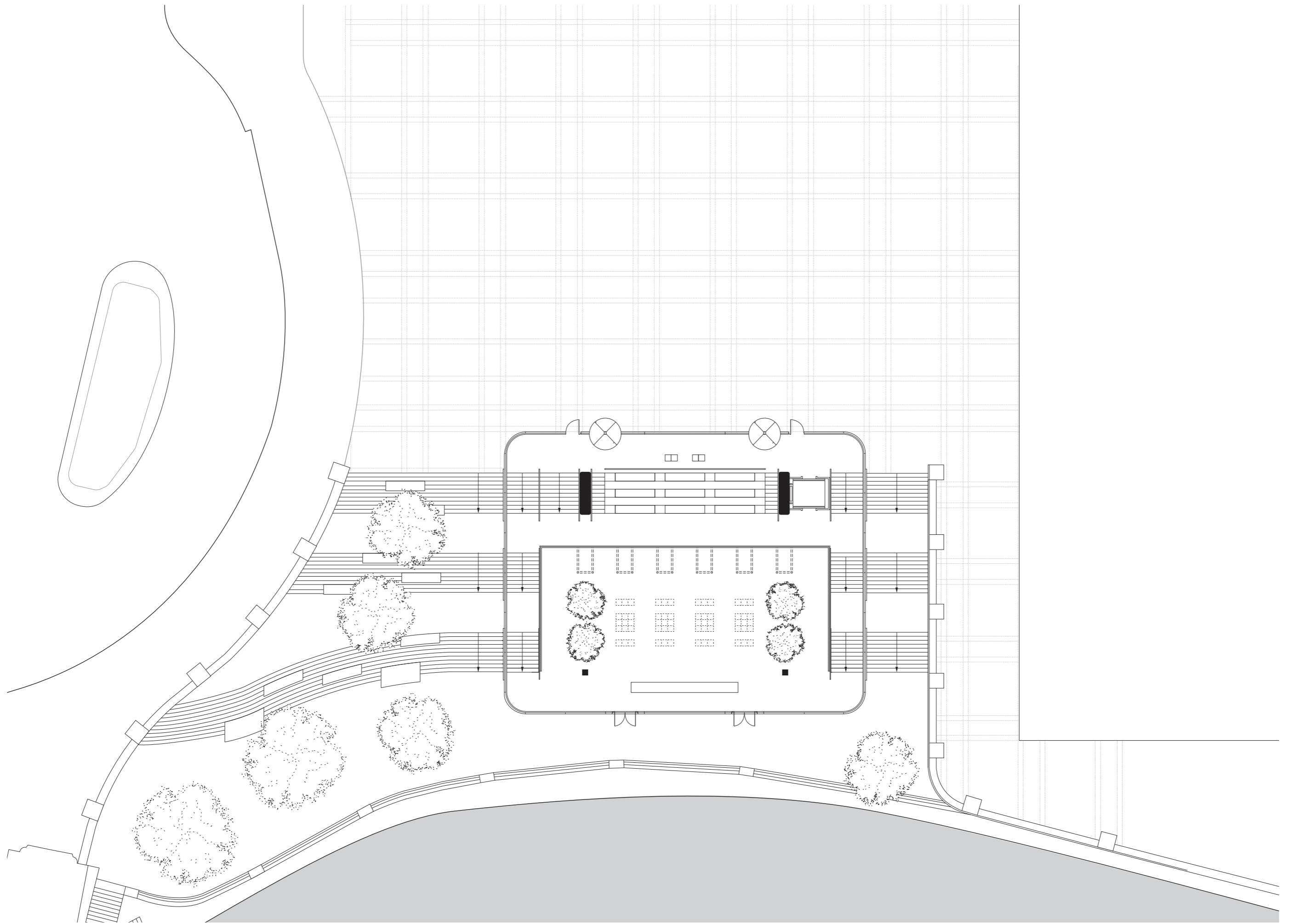
Mezzanine Level Plan
