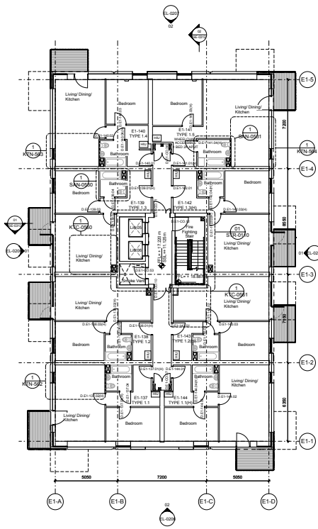
02 FLOOR 03 PLAN
