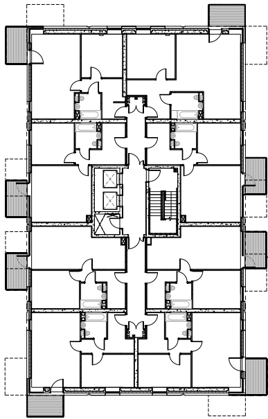
01 FLOOR 02 PLAN
