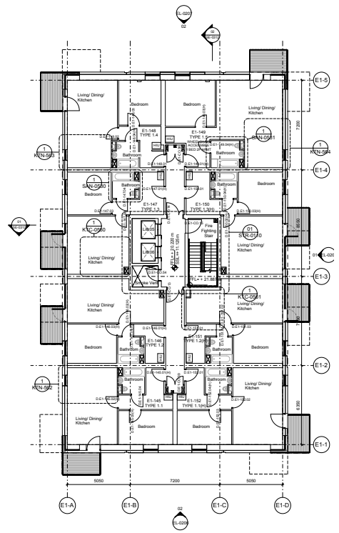
03 FLOOR 04 PLAN
