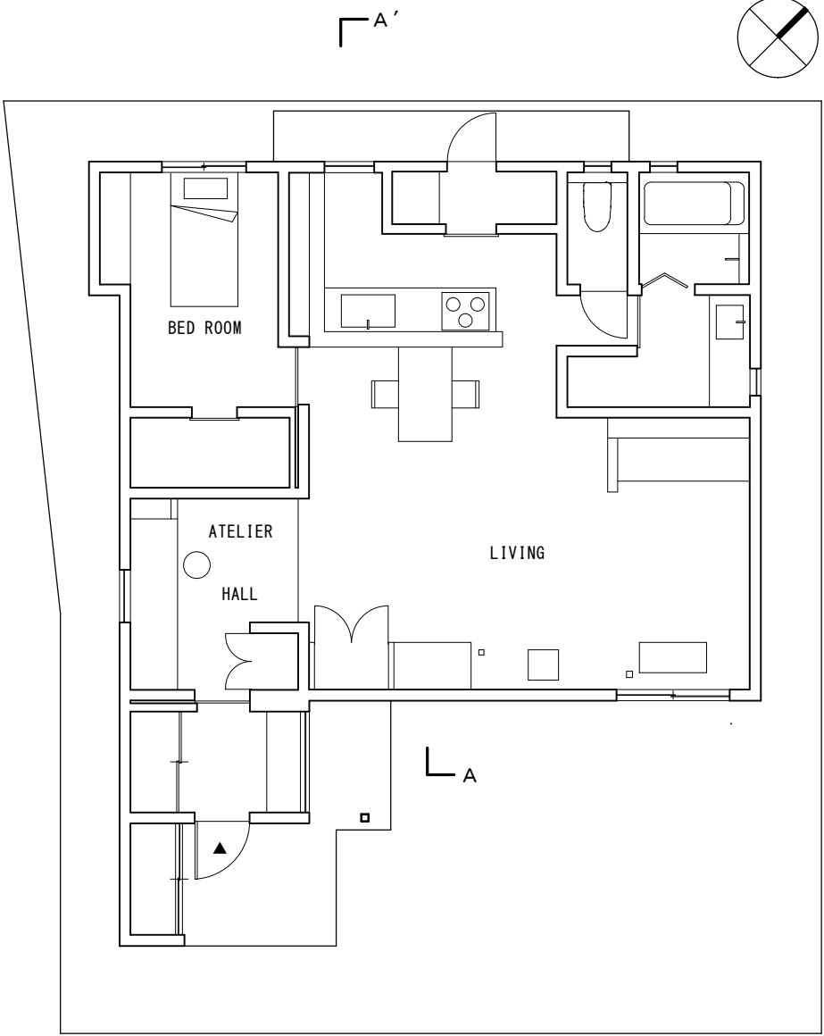
1F PLAN
