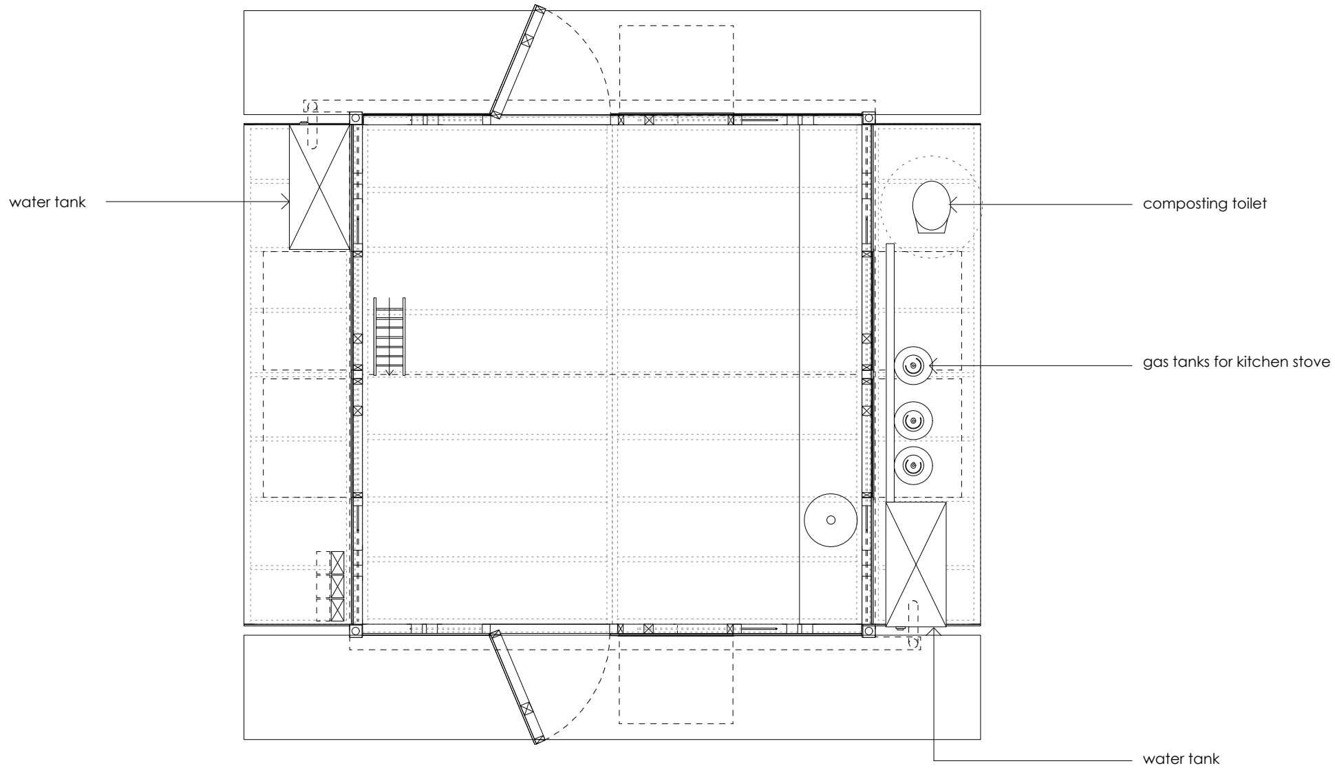
FLOOR PLAN
