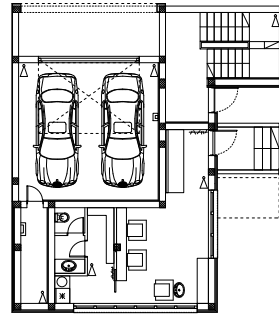
GROUND FLOOR
