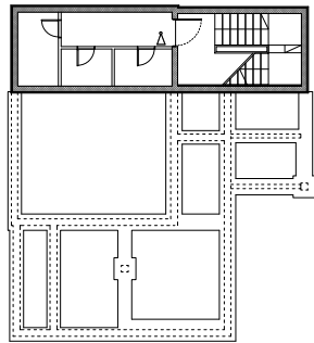
BASEMENT FLOOR
