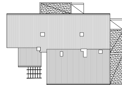
ROOF FLOOR
