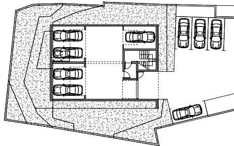
BASEMENT FLOOR
