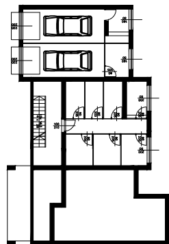
BASEMENT FLOOR
