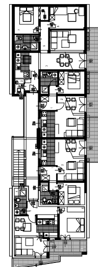
THIRD FLOOR
