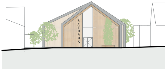
ELEVATION WEST
