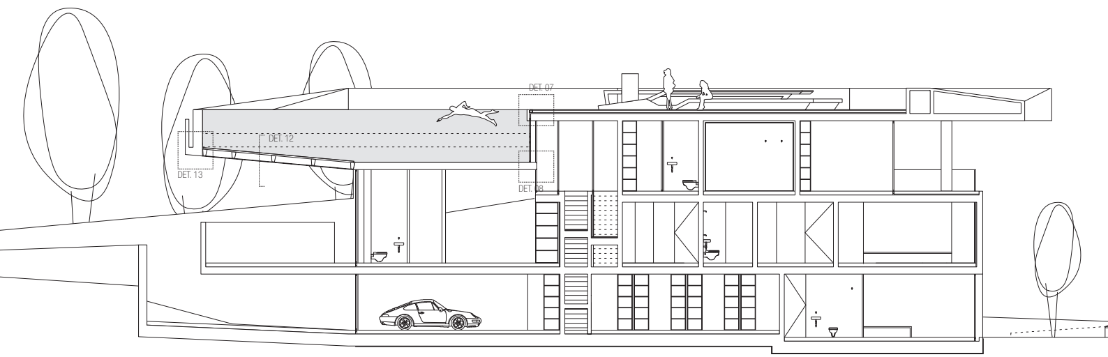
SECTION AA
