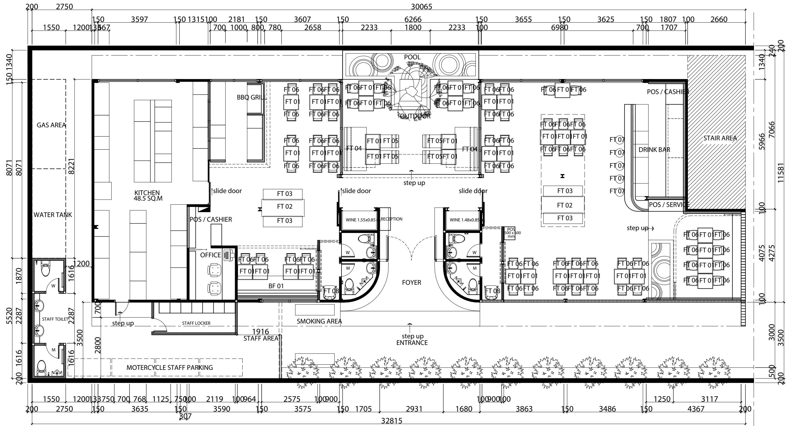
FURNITURE LAYOUT-00 scale 1:100 all units in millimetre
