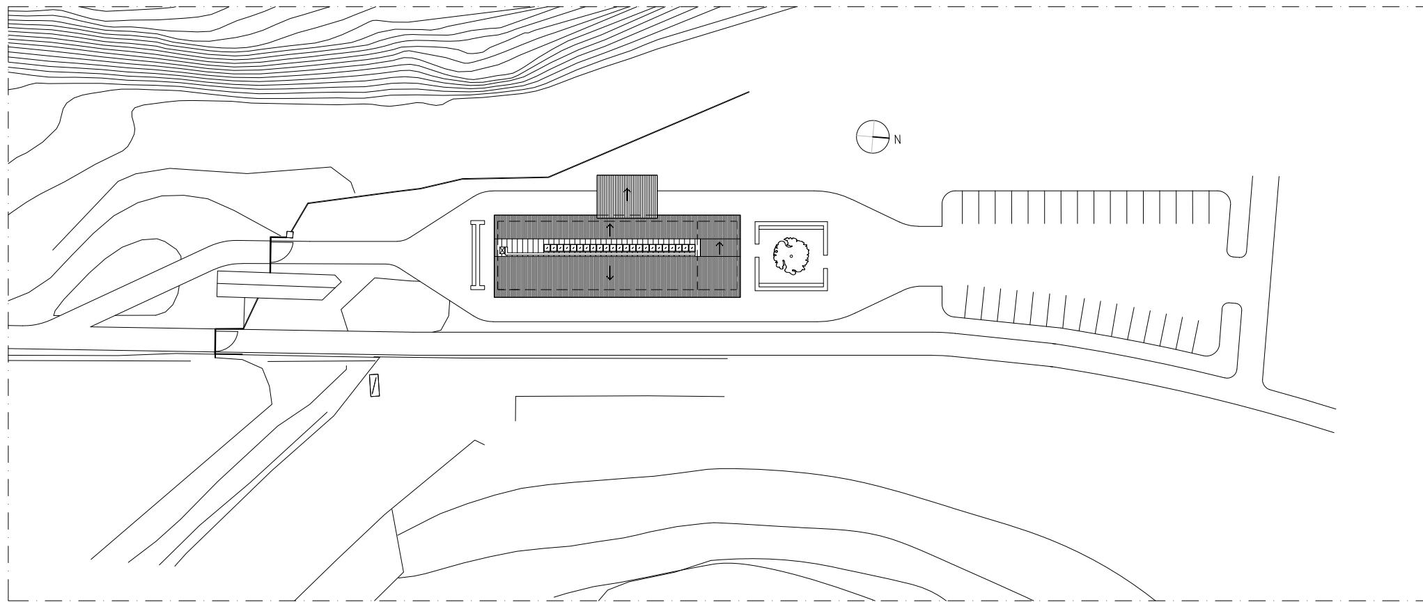
SITE LAYOUT PLAN Scale 1:400 (A1)
