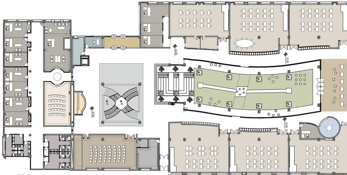
Ground floor plan (current situation)
