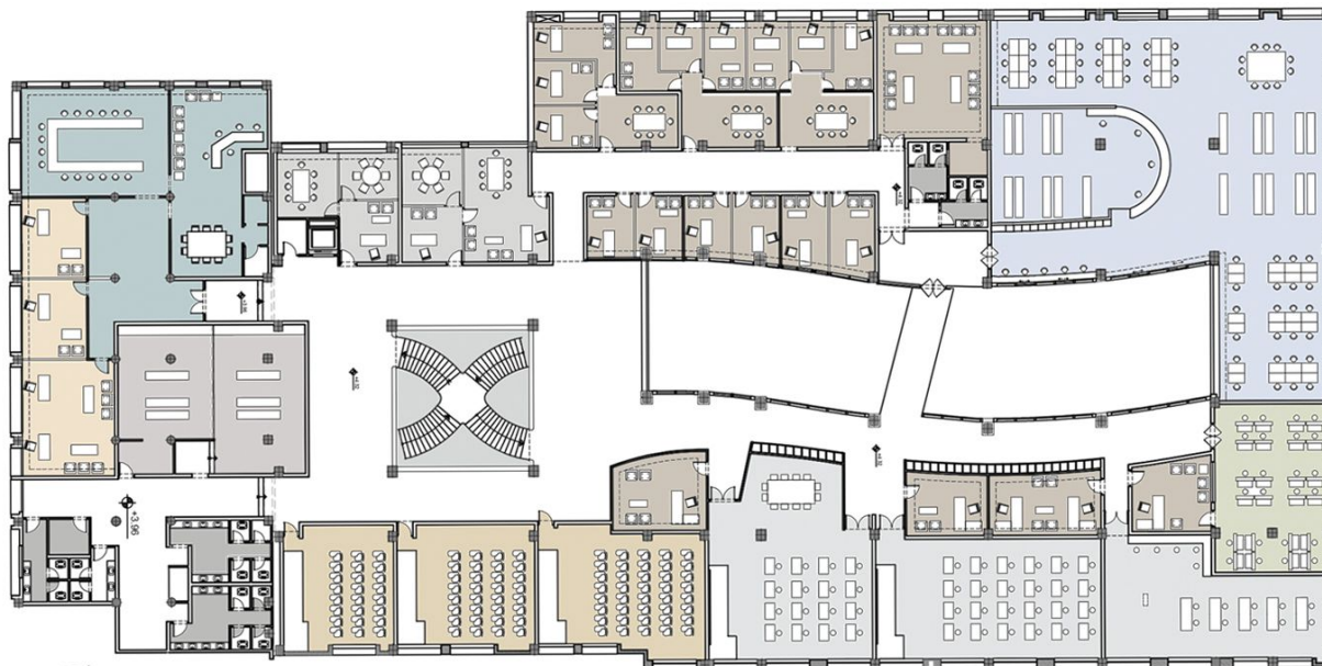
First floor plan (current situation)
