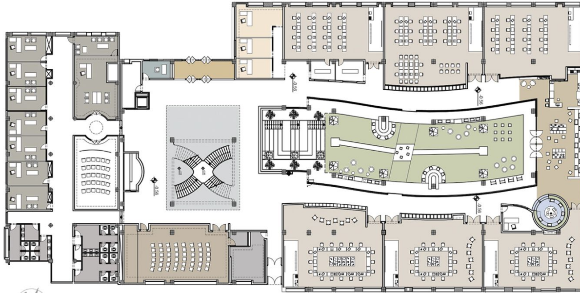
Ground floor plan (The best alternative)
